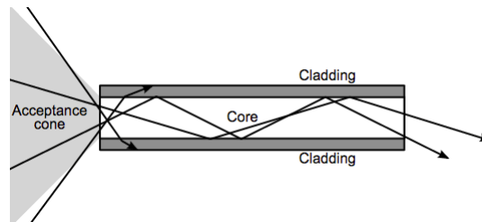
Figure 6: Optical fibre
